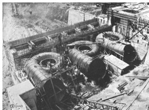
Construction work at Ardnacrusha
